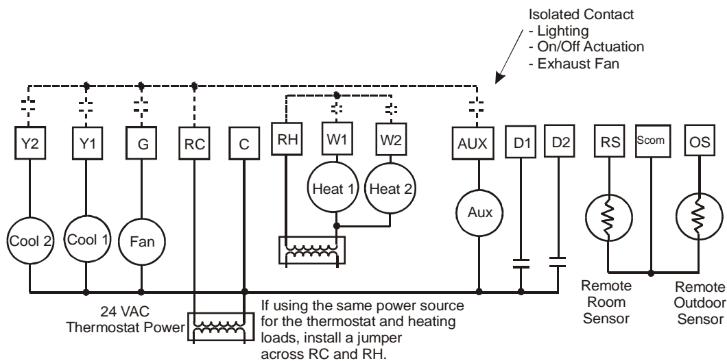
Figure 6: Wiring the T600MSx-3 Thermostats
