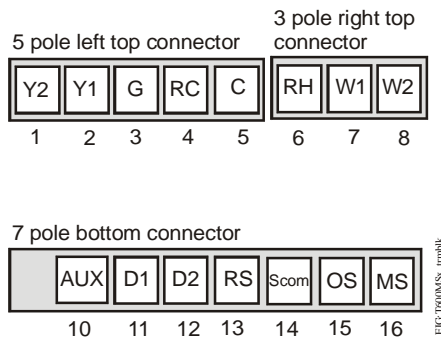
Figure 5: Terminal Blocks
